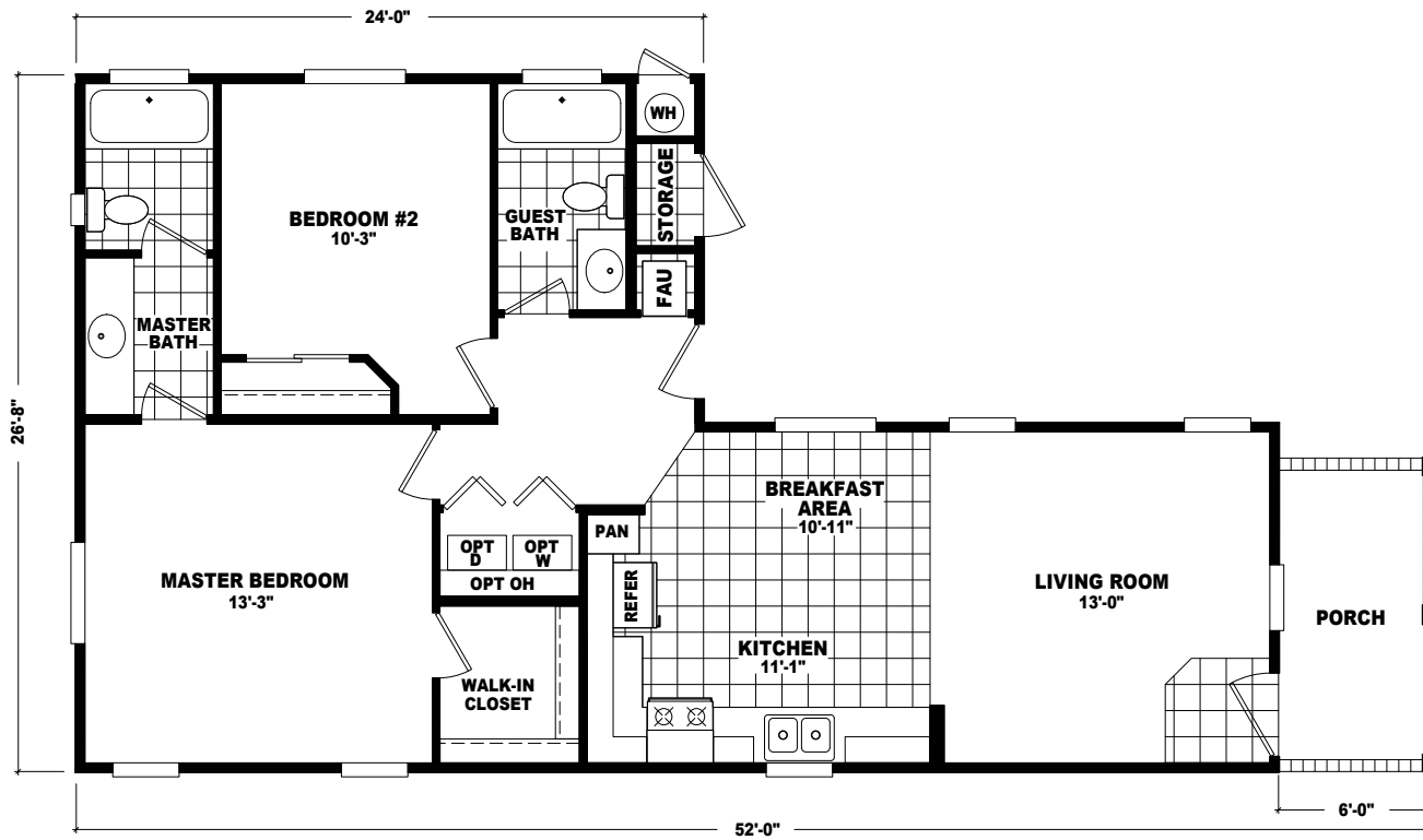
MODEL: VPH-2852A APPROXIMATELY 1005 SQ. FT. TOTAL APPROXIMATELY 933 SQ. FT. LIVABLE 2 BEDROOM, 2 BATH
