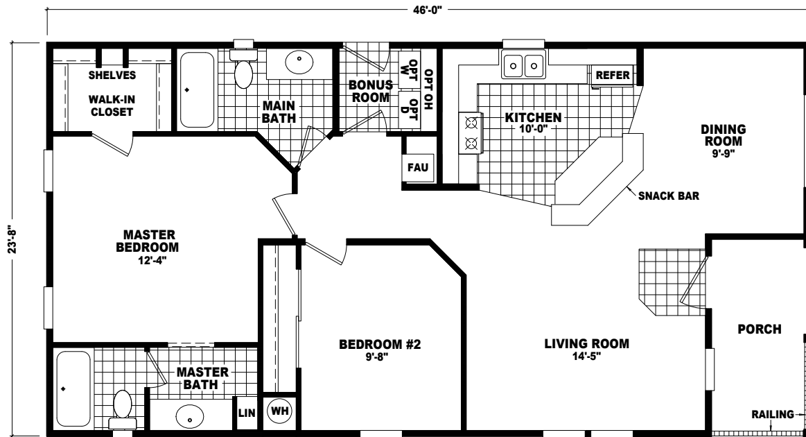
MODEL: VPH-2446A APPROXIMATELY 1088 SQ. FT.* 2 BEDROOM, 2 BATH *INCLUDES PORCH REVISED: 21JUN15 D
